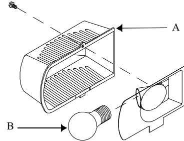
A. Light bulb cover
